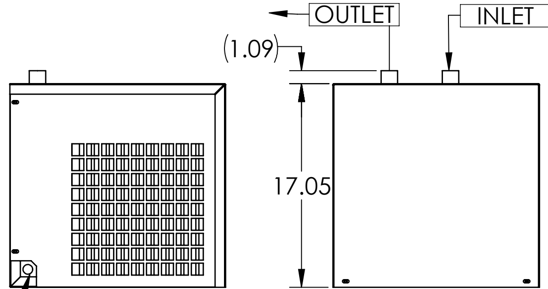
REAR VIEW
